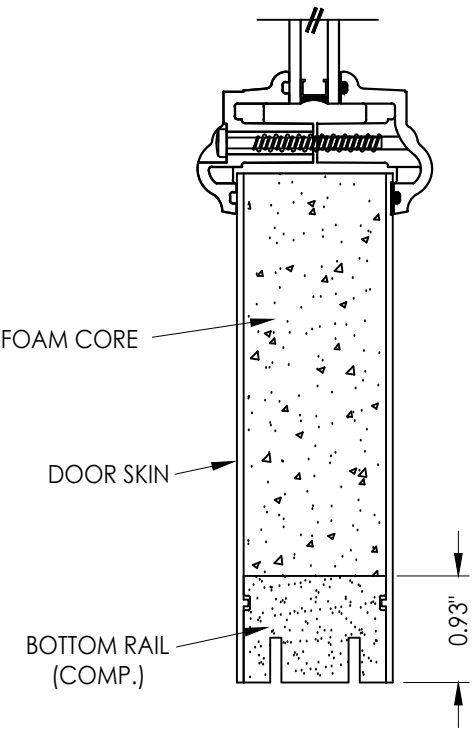
2 VERTICAL CROSS SECTION
