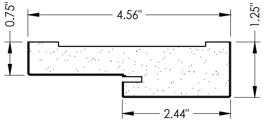
6 POLY FIBER TRANSOM JAMB
