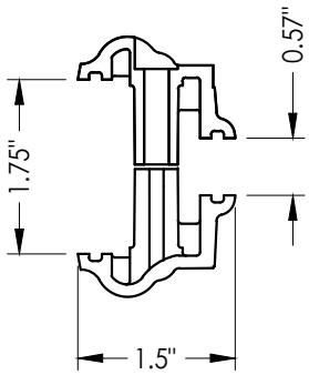
3A ODL LITE FRAME HP Polypropylene
