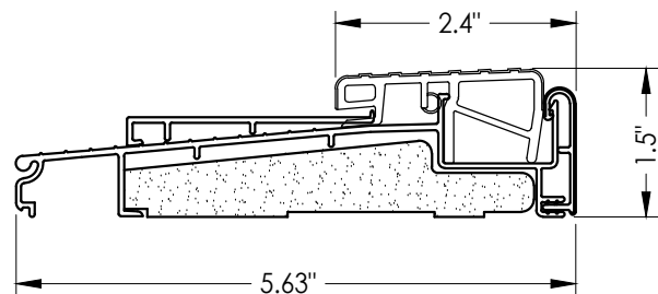
23 OUTSWING THRESHOLD w/ SIDELITE ADAPTER Endura (Z-Series)
