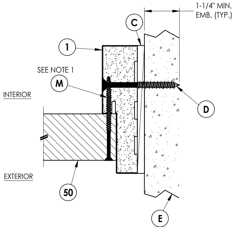
4 8 HORIZONTAL CROSS SECTION Outswing shown Direct to Masonry Construction
