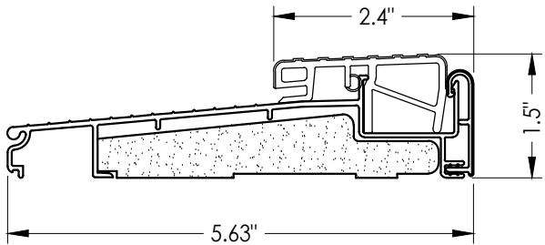
22 OUTSWING THRESHOLD Endura (Z-Series)
